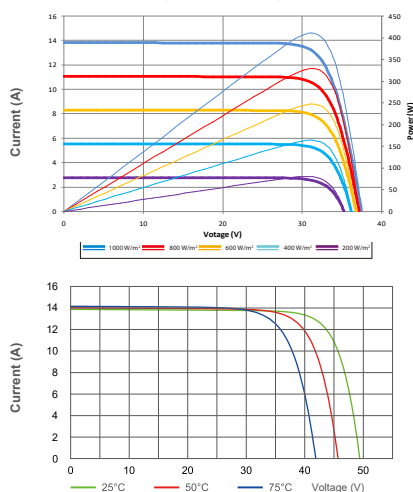
Current-Voltage &amp; Power-Voltage Curve (410)
